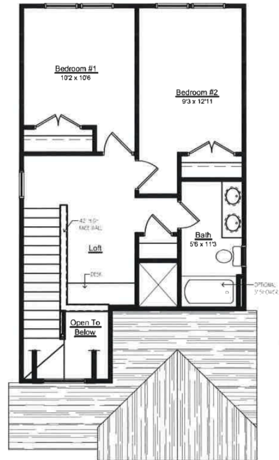
SECOND FLOOR STANDARD FLOOR PLAN
